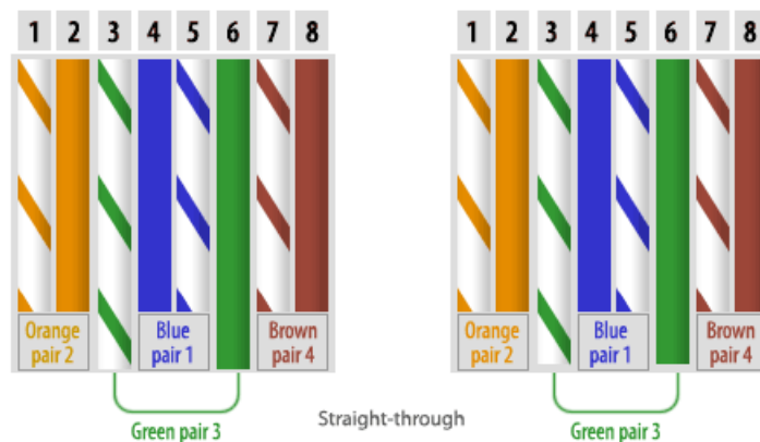
Gambar 1.8 Straight Cable
